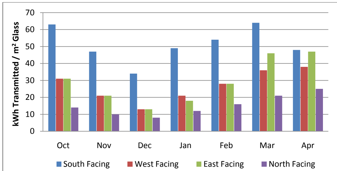
Figure 7: Solar gain for windows in the Halifax region as a function of orientation (Wood 2006)
